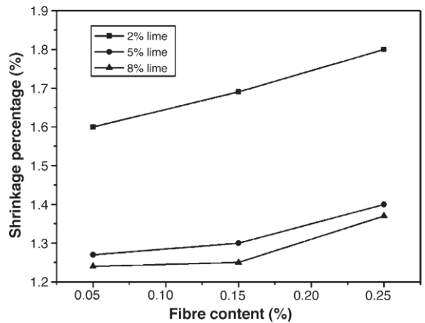
Fig. 5. Effect of the fibre content on shrinkage percentage of fibre–lime treated soil specimens after 7-day curing.
