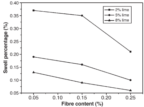
Fig. 4. Effect of the fibre content on swell percentage of fibre–lime treated soil specimens after 7-day curing.
