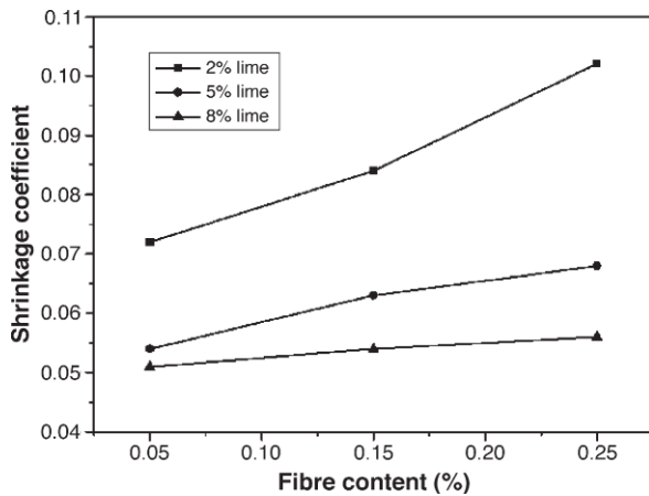
Fig. 6. Effect of the fibre content on shrinkage coefficient of fibre–lime treated soil specimens after 7-day curing.
